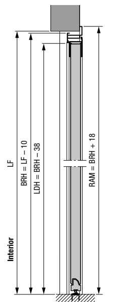
Side door with aluminium corner frame, profile type 2 External fitting
